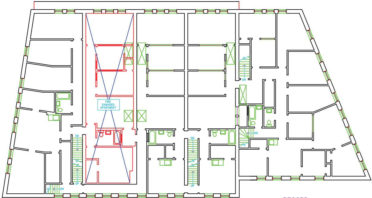
RECORD UPPER LEVEL PLAN SCALE: 3/16"=1'-0"
